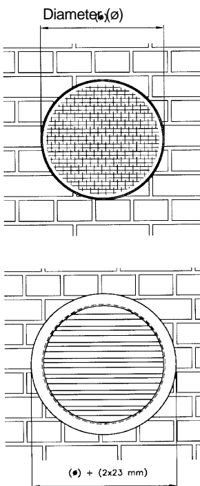
Diameter (ø) + (2 x 23 mm)
